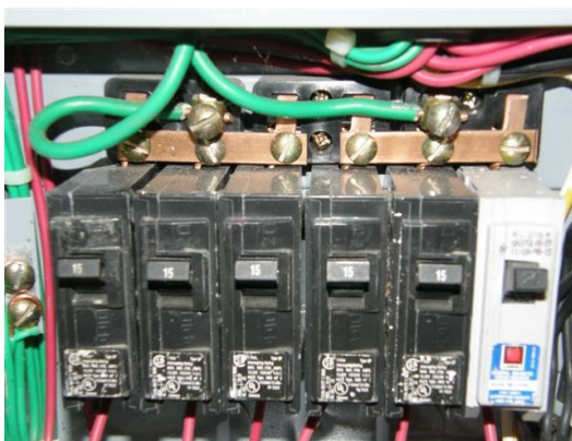
breaker
