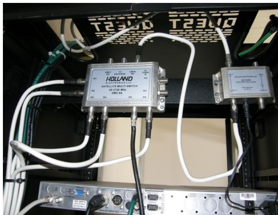
SPLITER PARABOLICA
