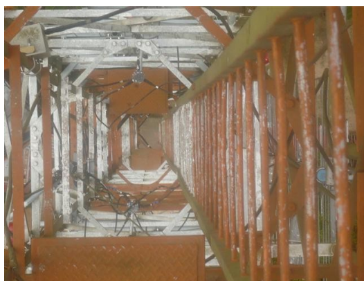
Escalerilla vertical
